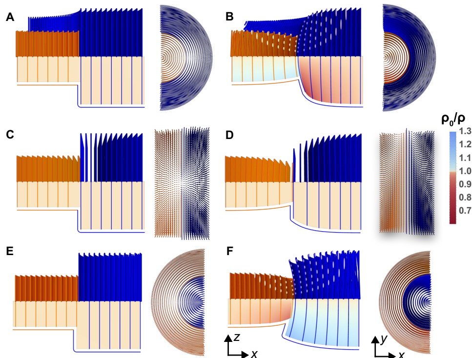
Fig. 2. Coupling between interface curvature, rod tilt, and density. (A and B) Structure of domain interface with curvature toward short rods ( \kappa_g < 0 ). Left: Side and top views show the constant rod density of an untwisted curved domain. Right: The same interface with rod twist shows a splayed structure and expansion of the short rods and compression of the long rods. (C and D) For interface without spontaneous curvature ( \kappa_g = 0 ), the rod density is constant whether rods are straight or tilted. (E and F) When \kappa_g > 0 , rod density around the untwisted interface again remains constant, while rod twist leads to expansion of the long and compression of the short rods.
